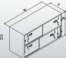
4 CURRENCY BIN CABINET / 4 CURRENCY BIN CABINET (SPL.)
